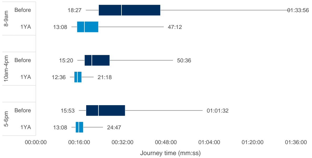
Figure 9: Changes in southbound journey time reliability
