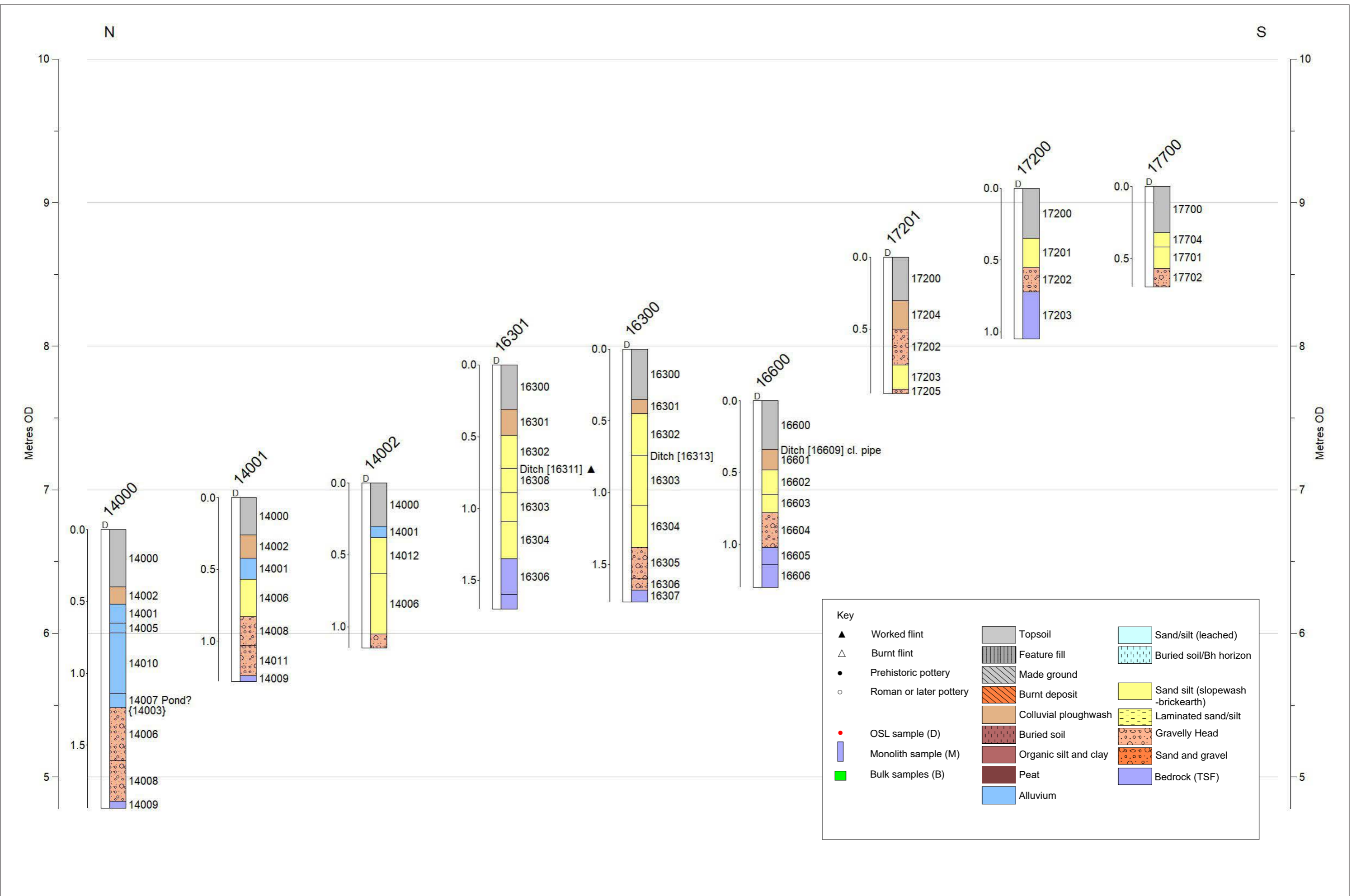
Figure 57: Geoaerchaeological Transect 12: Trenches 140, 163, 166, 172 and 177
