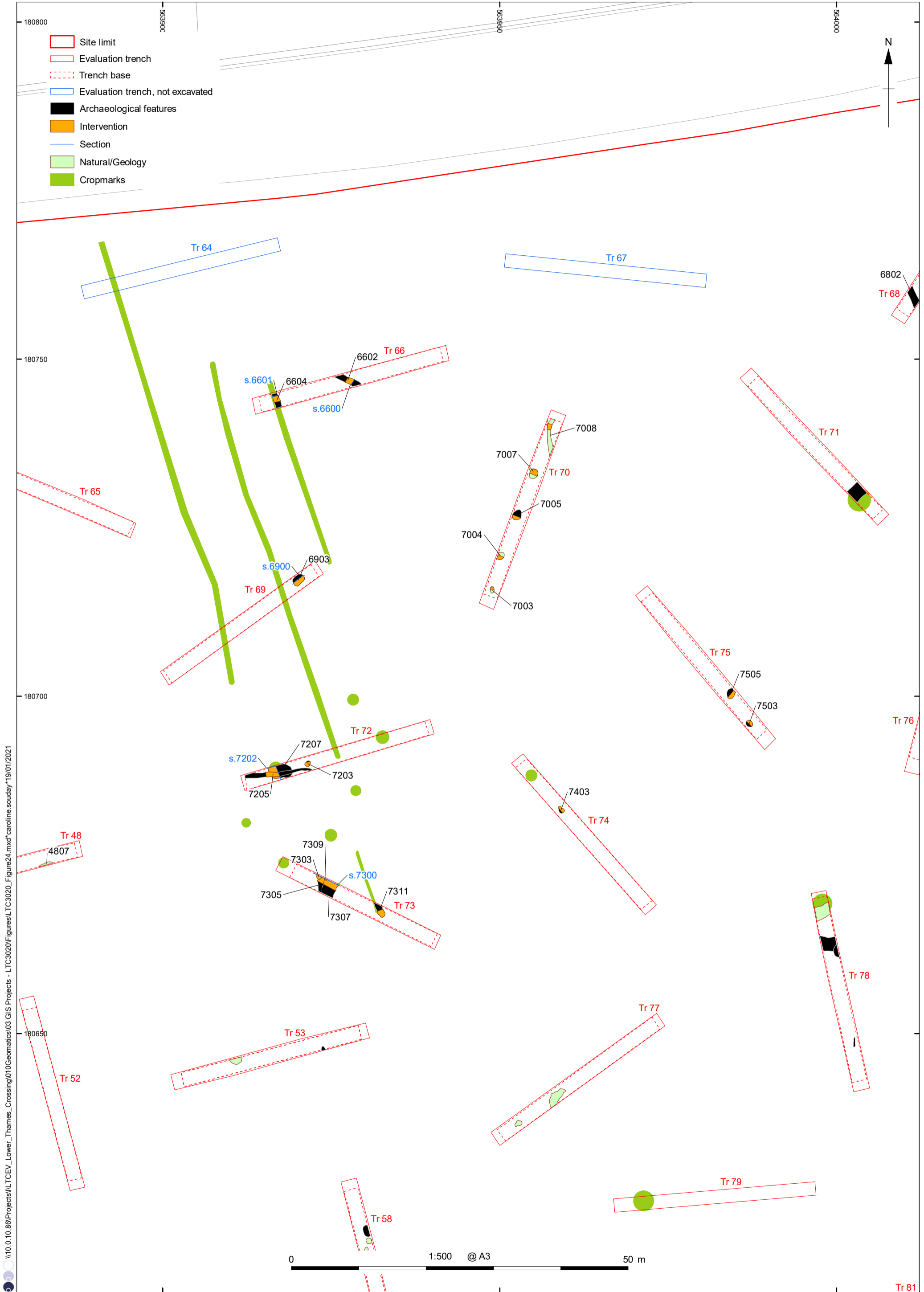
Figure 24: Detailed plan of Trenches 66, 69, 70 and 72-5
